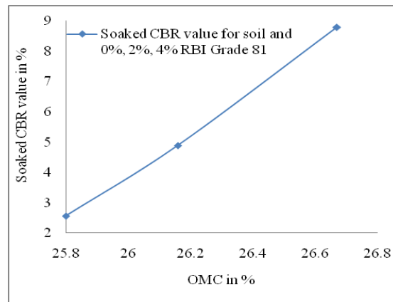
Fig.2. Effect of RBI Grade 81 on CBR and OMC of soil
