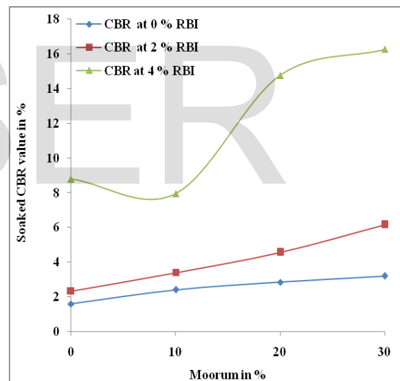
Fig.4. Effect of RBI Grade 81 and Moorum on CBR value of soil
