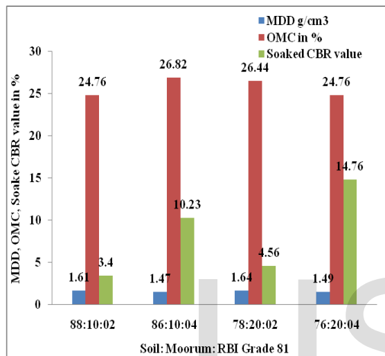
Fig.3. Effect of moorum and RBI Grade 81 on MDD, OMC and CBR value of soil
