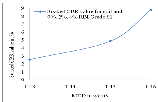
Fig.1. Effect of RBI Grade 81 on CBR and MDD of soil
